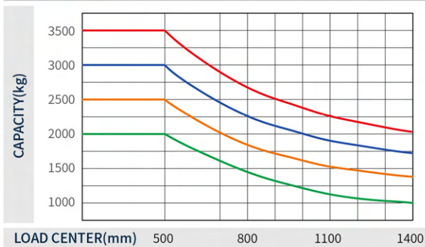
Load curve
