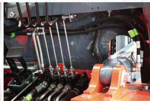
Large diameter hydraulic pipe, Standard 24 degrees conical seal.
